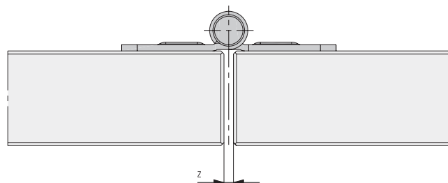
Variante 1, paumelle plate : Z = 1-6mm
