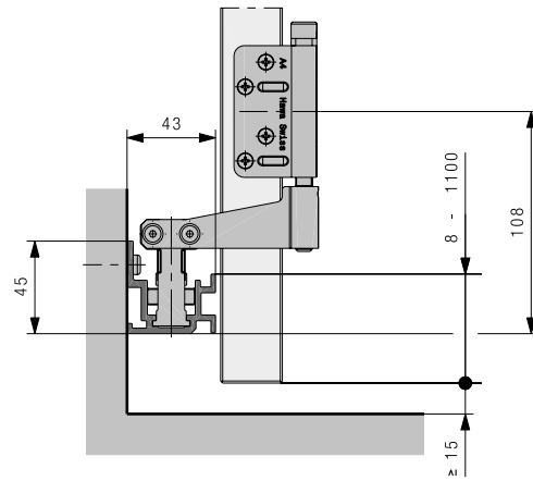
Rail de guidage montage mural
